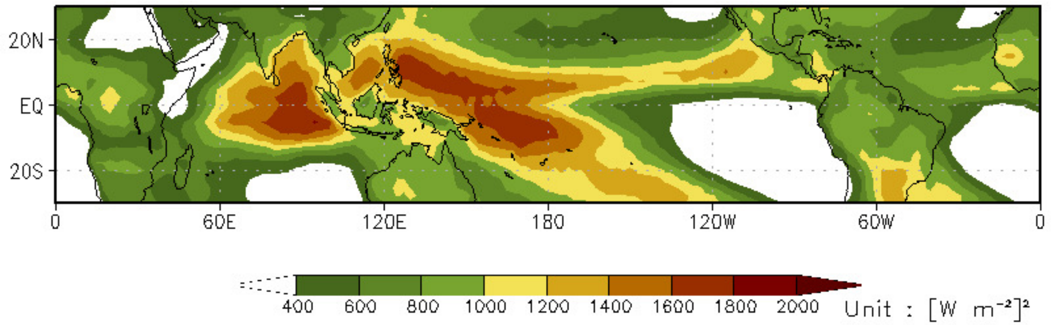
(a) Unfiltered variance, OLR, AVHRR, All season
