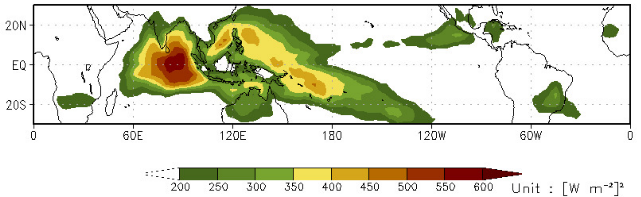
(b) 20–100 day variance, OLR, AVHRR, All season
