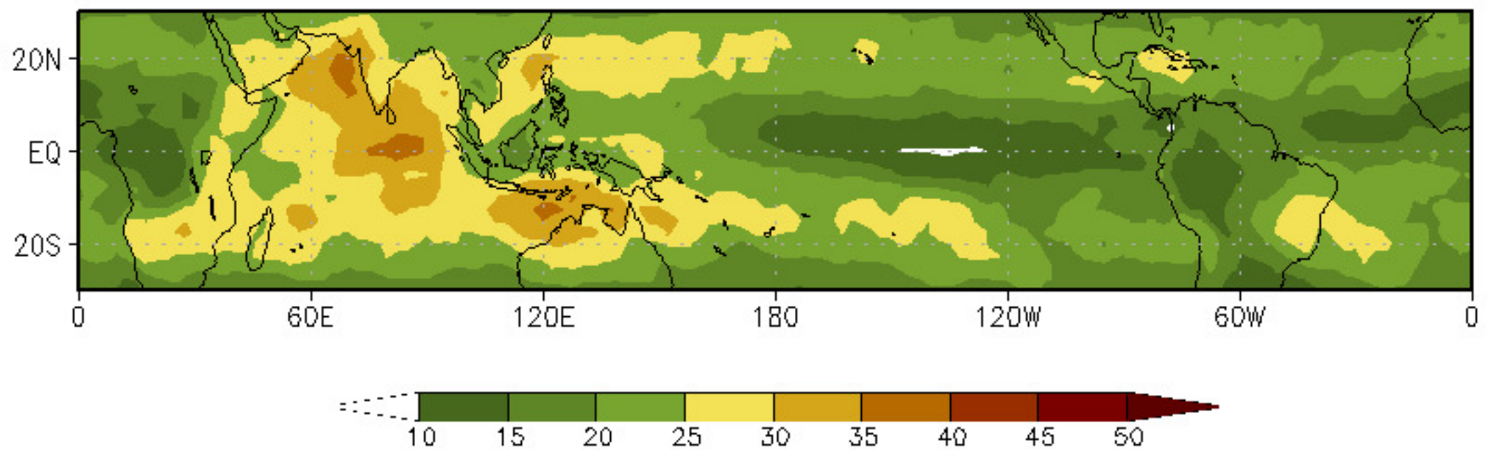
(c) % of Unfiltered variance, OLR, AVHRR, All season
