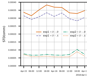
(e) bending angle (rad) @ SPol
