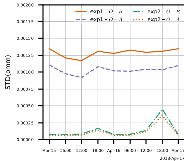
(c) bending angle (rad) @ Tro
