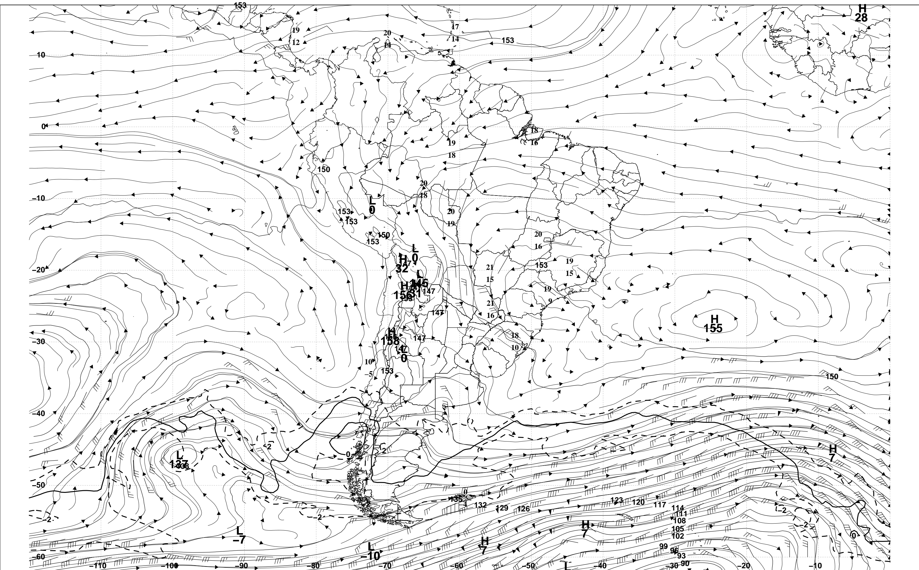
240423/0000 850 MB BRBK:1.5:2:112 TMPC DWPC 240423/0000V000 850 MB WIND (KTS), AND HEIGHT
