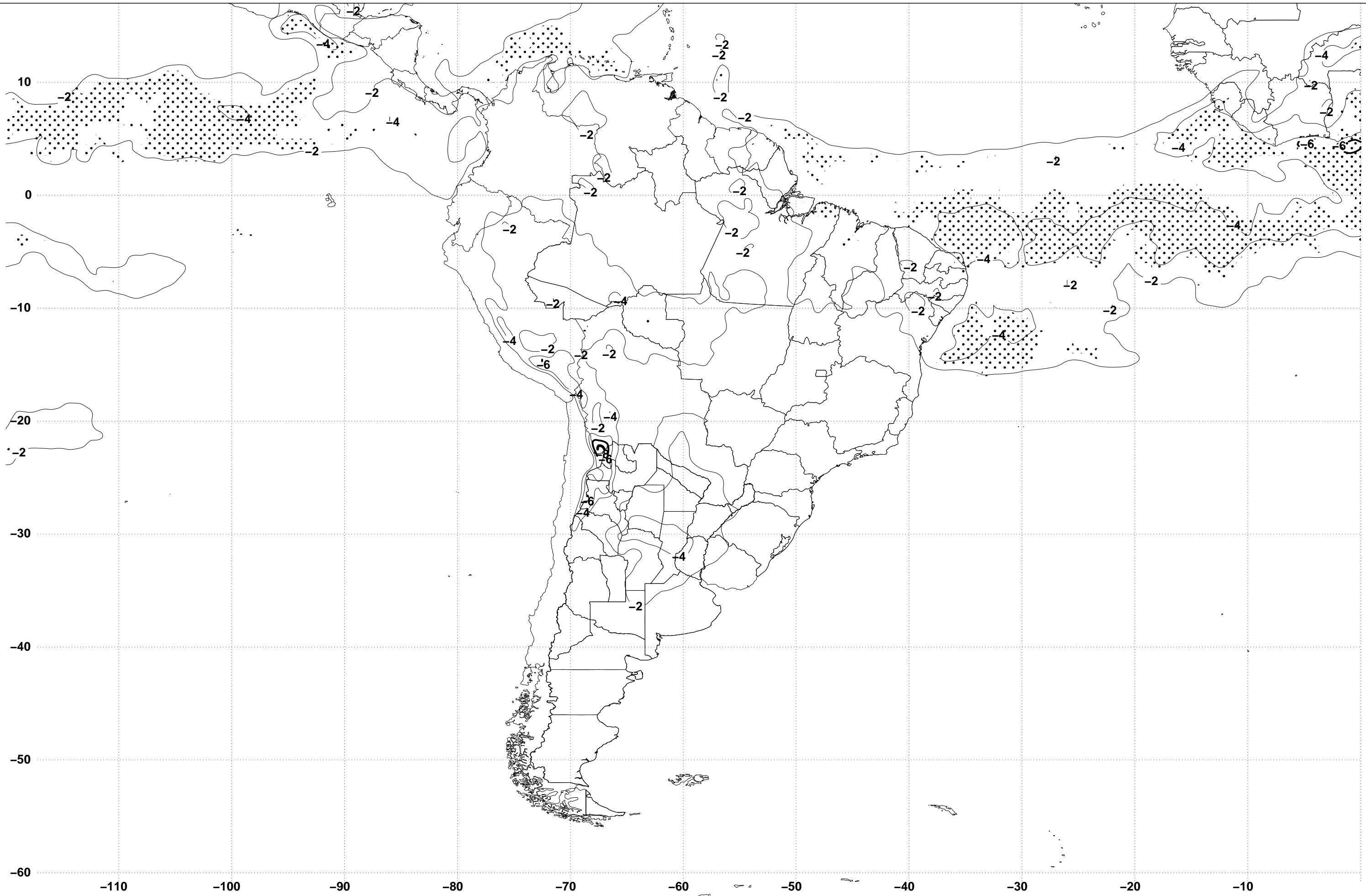
240422/1200V000 CAPE (somb; > 1000) AND LFT4 (cont)
