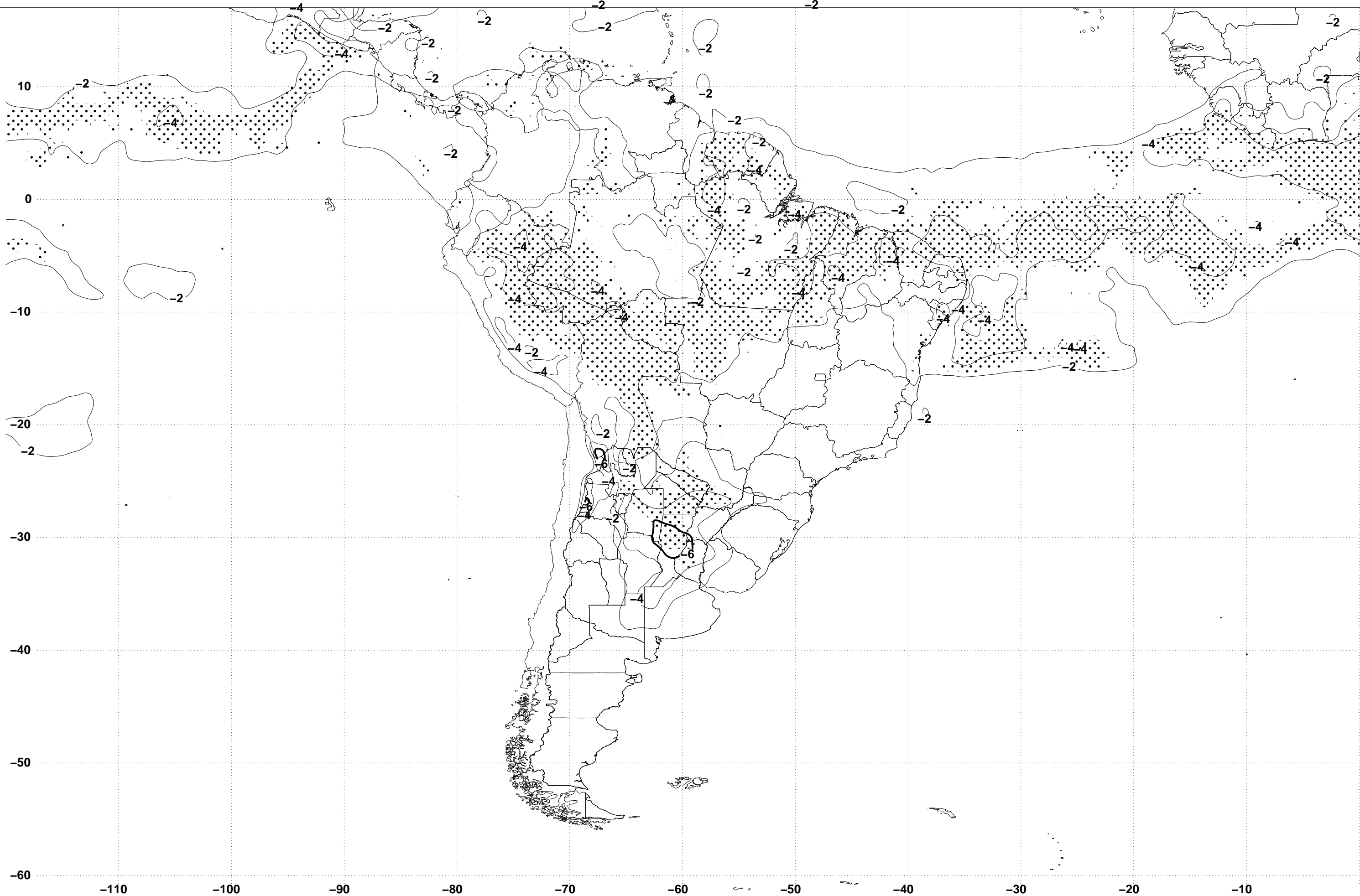
240422/1800V00 CAPE (somb; > 1000) AND LFT4 (cont)
