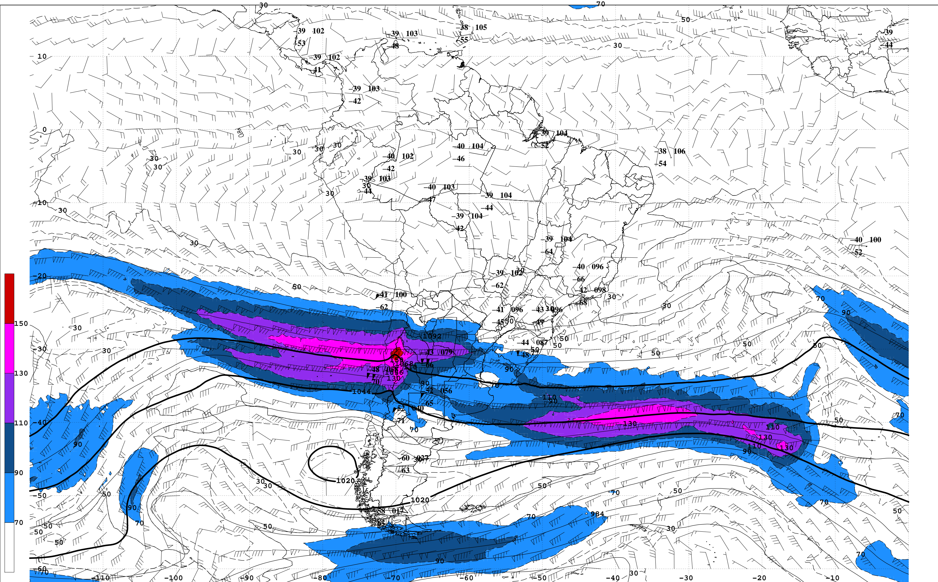
240422/1200 250 MB BRBK:1:2:T12 TMPC STDZ DWPC
